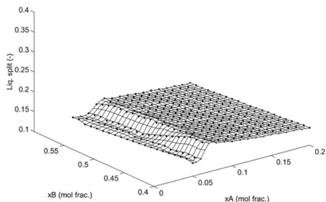
Fig. 5. Surface plot of liquid split ratio to the prefractionator with different liquid compositions at one stage above feed tray in the BTX process.
