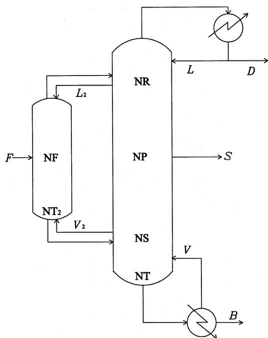
Fig. 1. A schematic diagram of a fully thermally coupled distillation column.
