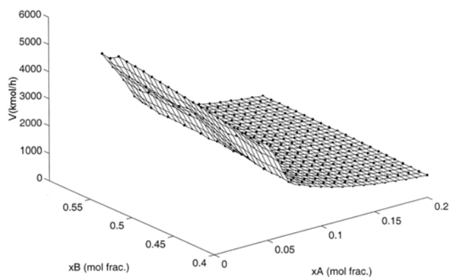
Fig. 3. Surface plot of vapor flow rates with different liquid compositions at one stage above feed tray in the BTX process.
