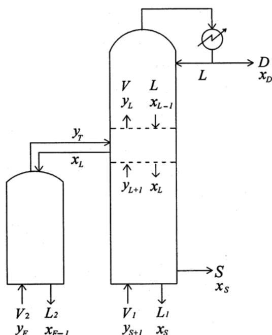
Fig. 2. A schematic diagram of top segment of the fully thermally coupled distillation column for the formulation of material balances calculating operational variables.
