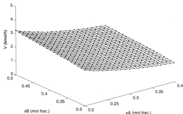
Fig. 4. Surface plot of vapor flow rates with different liquid compositions at one stage above feed tray in the butanol process.
